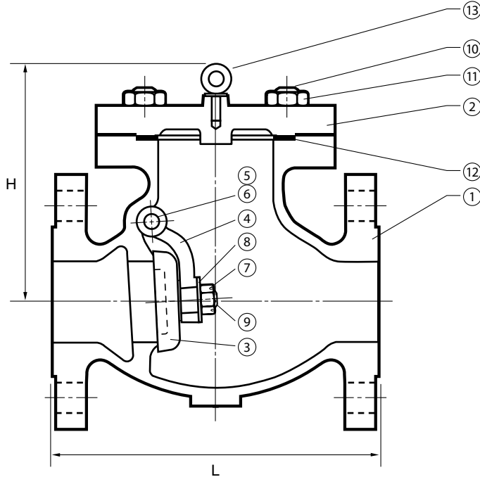
FIG 45B-150-CF8M (316 SS) FIG 45L-150-CG8M (317 SS)
